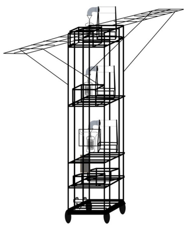
Tampak kiri
