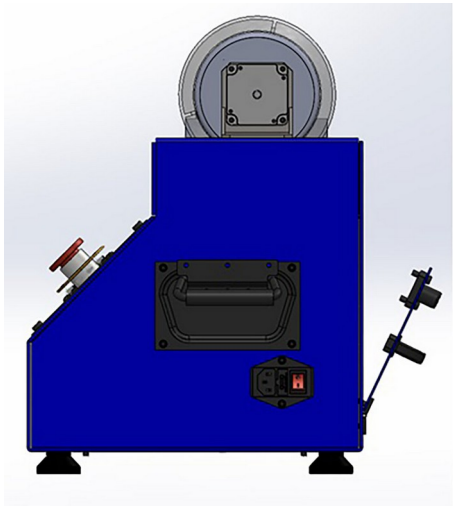
Tampak Samping
