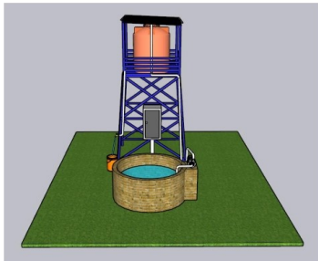
Tampak Samping Kiri
