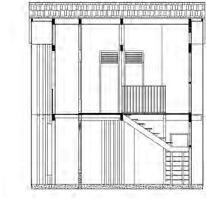
Tampak Samping
