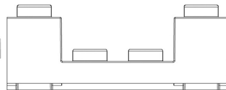
Tampak Samping
