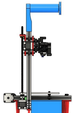
Tampak Samping
