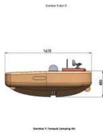
Tampak Samping
