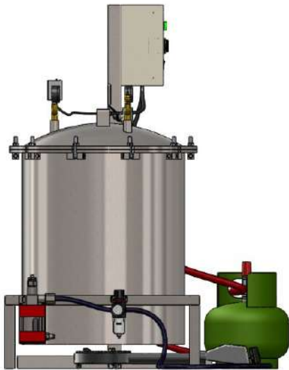
Tampak Samping
