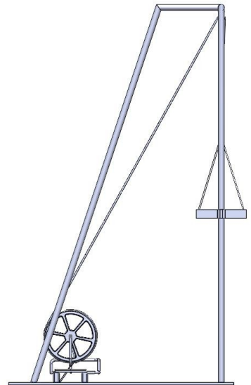
Tampak Samping
