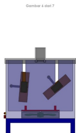
Gambar 6 : Tampak Samping Kiri
