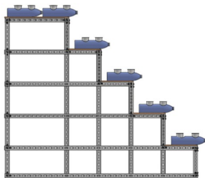
Tampak Samping
