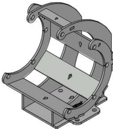
ISOMETRY VIEW
