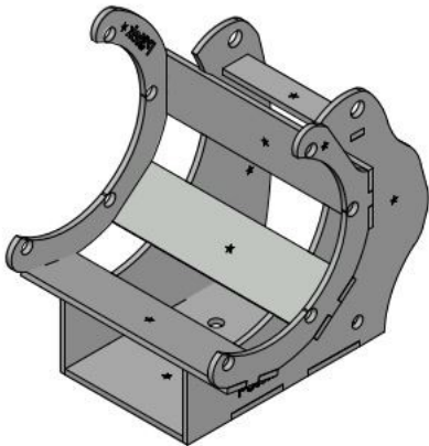
ISOMETRY VIEW
