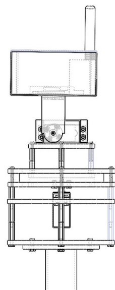
Tampak Samping
