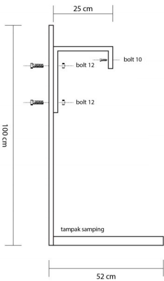
Tampak Samping
