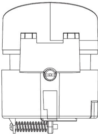
Tampak Samping
