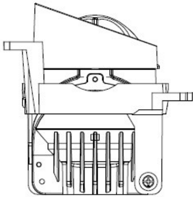
Tampak Samping
