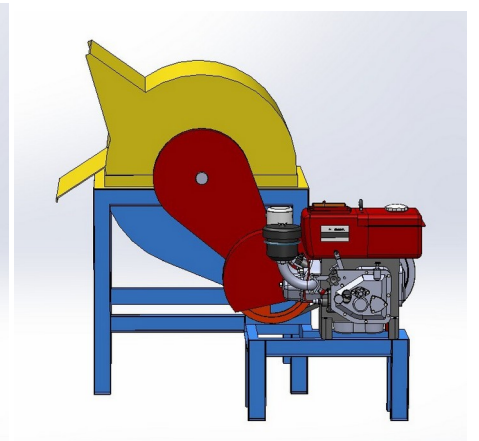
Tampak Samping
