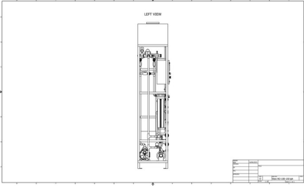
Tampak Samping
