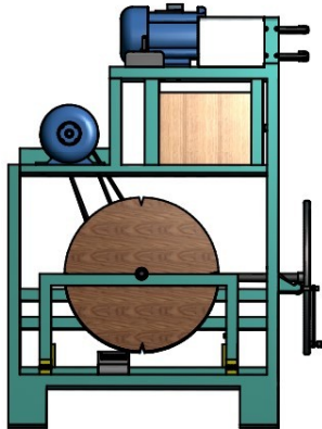
Tampak Samping
