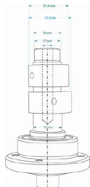
Tampak Samping
