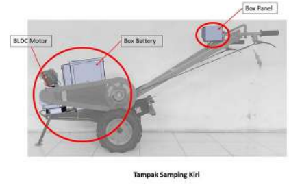
Tampak Samping
