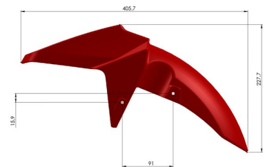
GAMBAR 6. TAMPAK SAMPING KIRI
