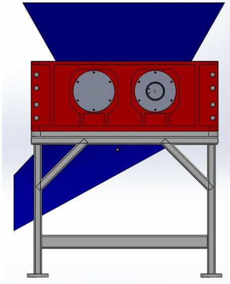
Tampak Samping
