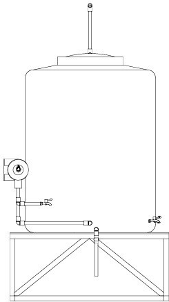
Tampak Samping
