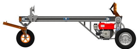
Tampak Samping
