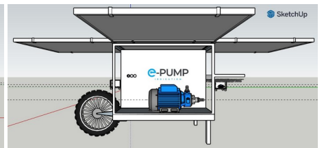
Tampak Samping
