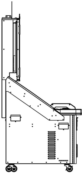
Tampak Samping
