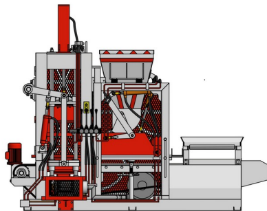
Tampak Samping
