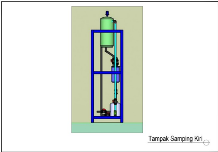
Tampak Samping
