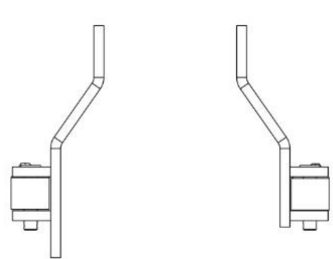
Tampak Samping
