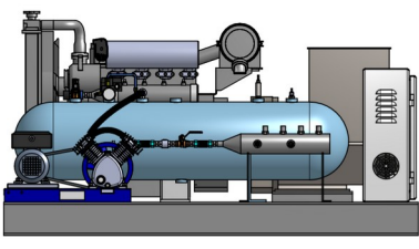
Tampak Samping
