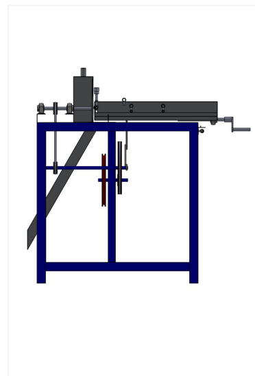
Tampak Samping
