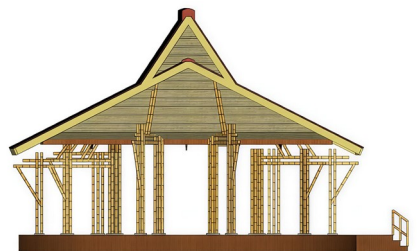
Tampak Samping
