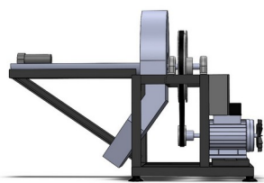
Tampak Samping
