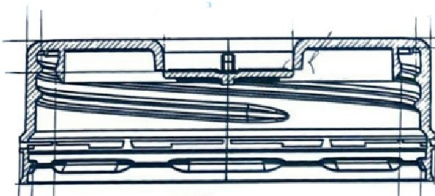
Tampak Samping
