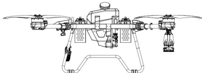
Tampak Samping
