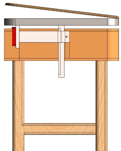
Tampak Samping
