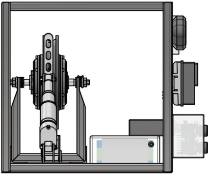
Tampak Samping
