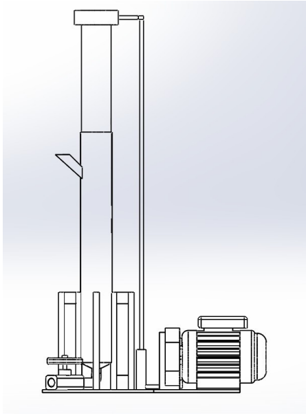
Tampak Samping
